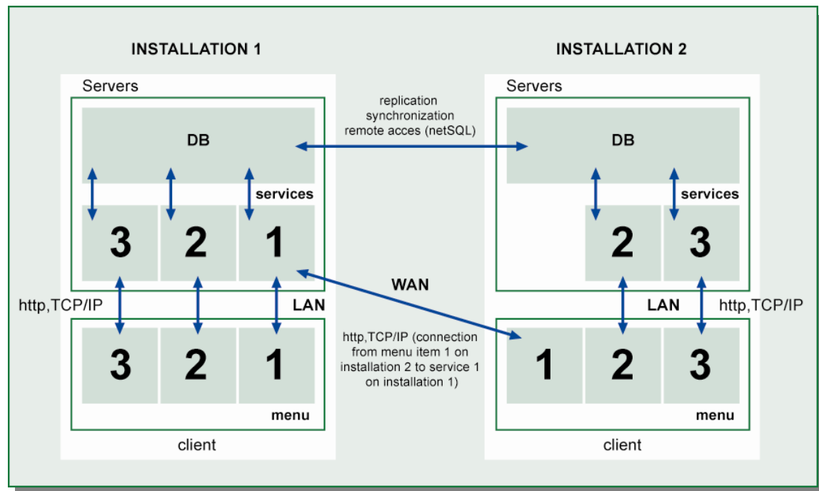
Figure 4.3 Optional Sharing of Services between Installations
