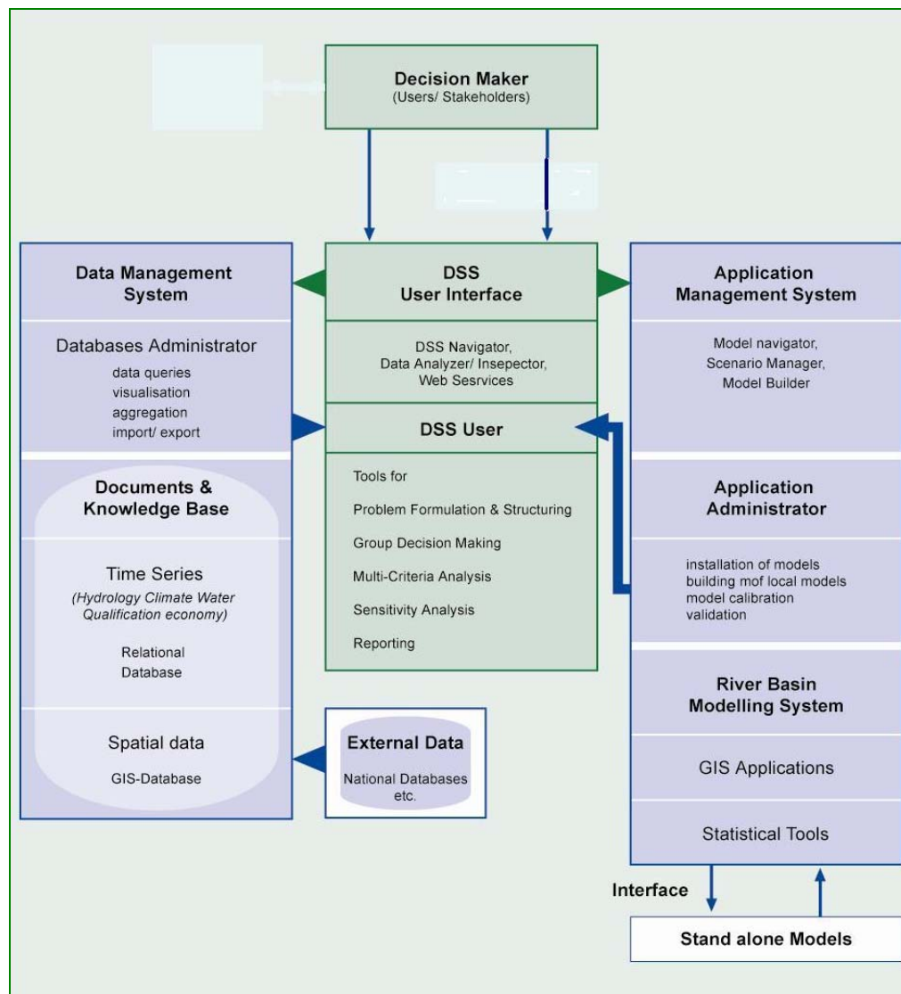
Figure 4.1 The Basic Components of the Nile-DSS
