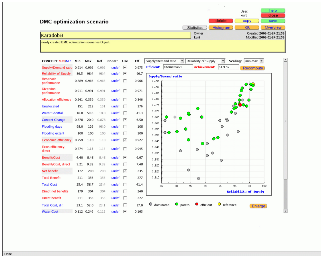
Figure 4.4 Scattergram of Alternatives on two Criteria Axes, normalized between NADIR and UTOPIA, showing dominated (grey) and efficient Solutions (red)
