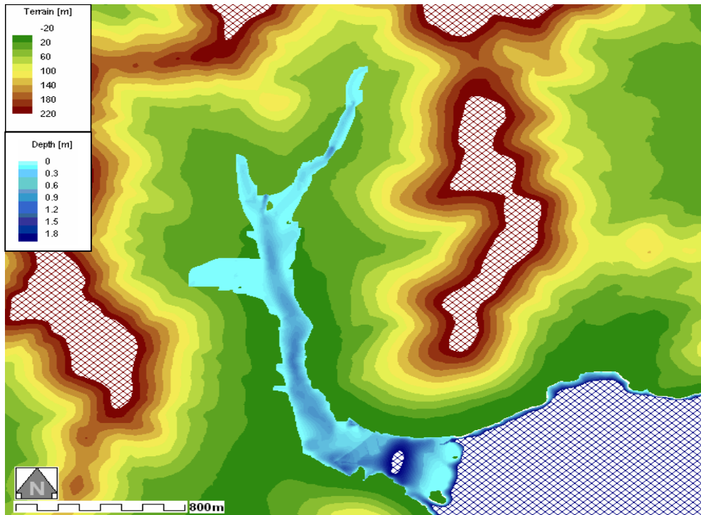
Figure 1: Water depth-Smooth DTM5_M20 in Terrain amp
