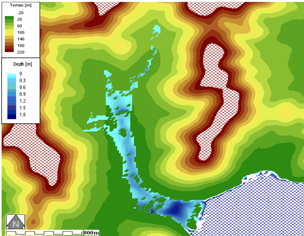
Figure 20: Water depth-Smooth with Roads and Buildings_DTM20_M20 in Terrain map
