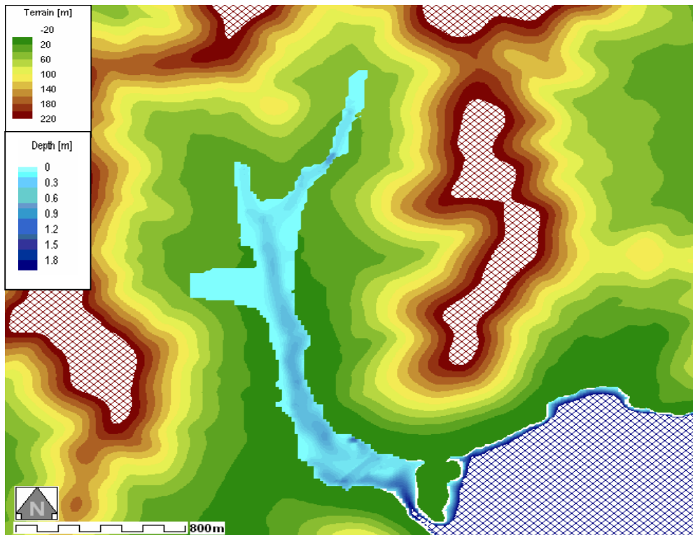
Figure 7: Water depth-Smooth DTM15_M30 in Terrain map
