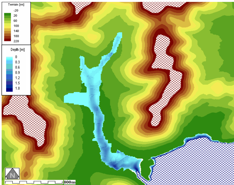
Figure 10: Water depth-Smooth with Roads_DTM10_M20 in Terrain map
