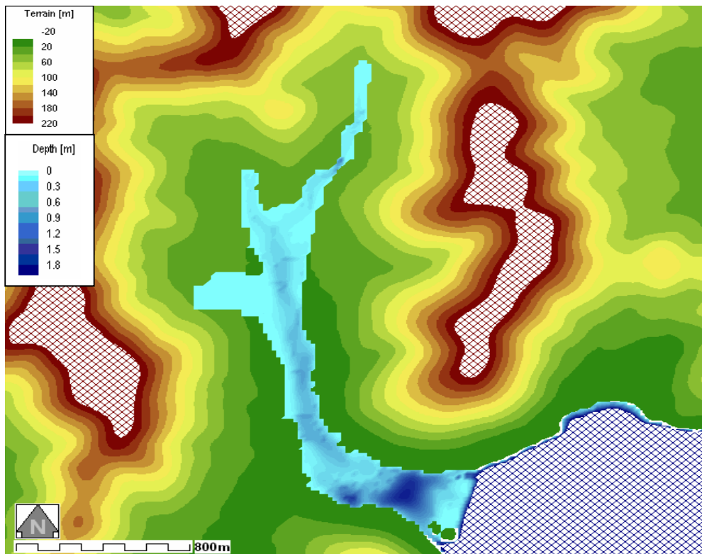
Figure 16: Water depth-Smooth with Roads_DTM20_M30 in Terrain map
