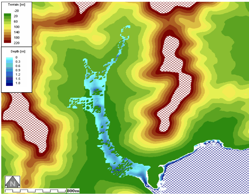
Figure 19: Water depth-Smooth with Roads and Buildings_DTM15_M20 in Terrain map
