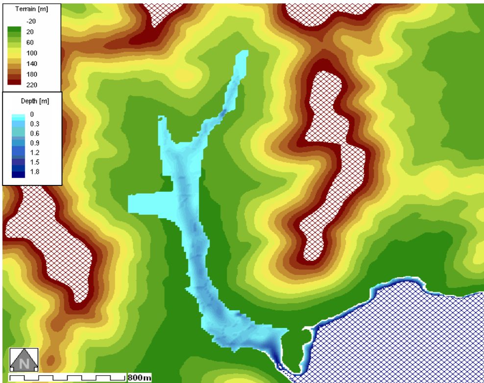
Figure 11: Water depth-Smooth with Roads_DTM15_M20 in Terrain map
