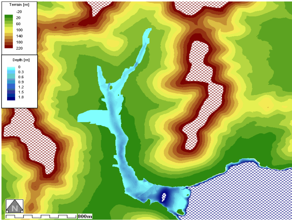
Figure 5: Water depth-Smooth DTM5_M30 in Terrain map
