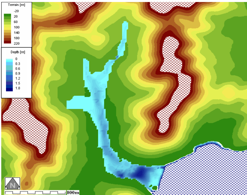
Figure 12: Water depth-Smooth with Roads_DTM20_M20 in Terrain map
