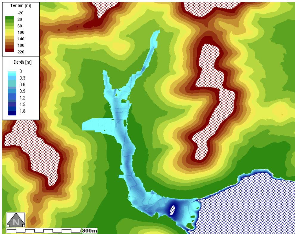
Figure 9: Water depth-Smooth with Roads_DTM5_M20 in Terrain map
