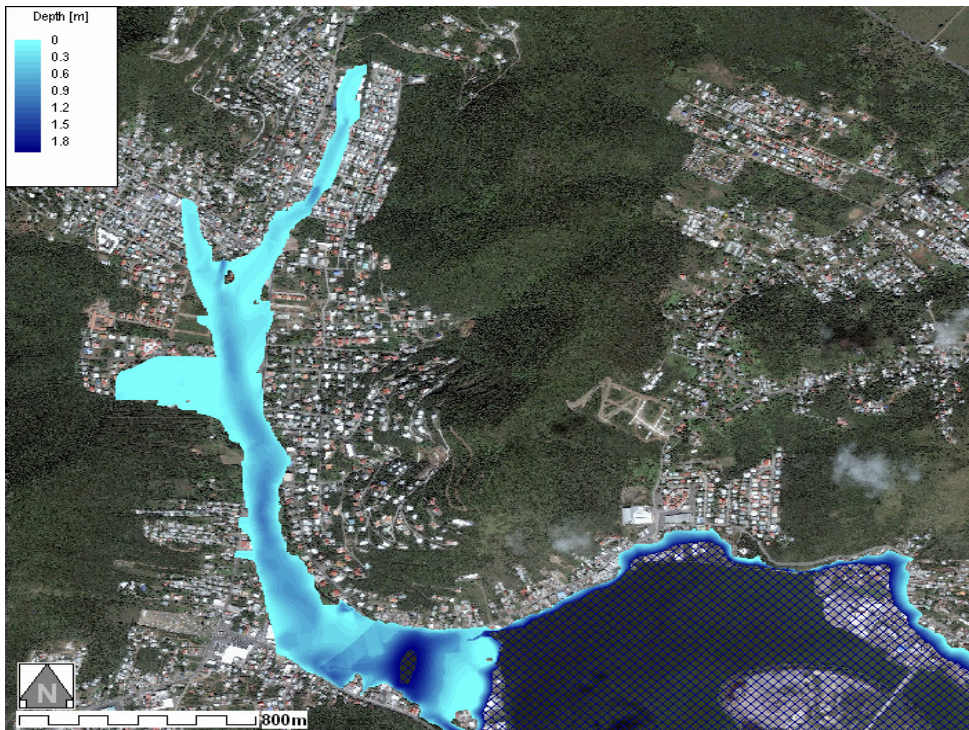
Figure 1: Water depth-Smooth DTM5_M20 Aerial Photo
