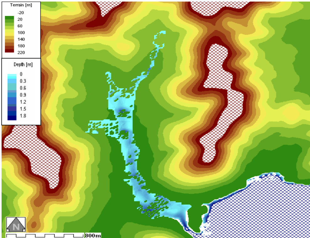
Figure 23: Water depth-Smooth with Roads and Buildings_DTM15_M30 in Terrain map
