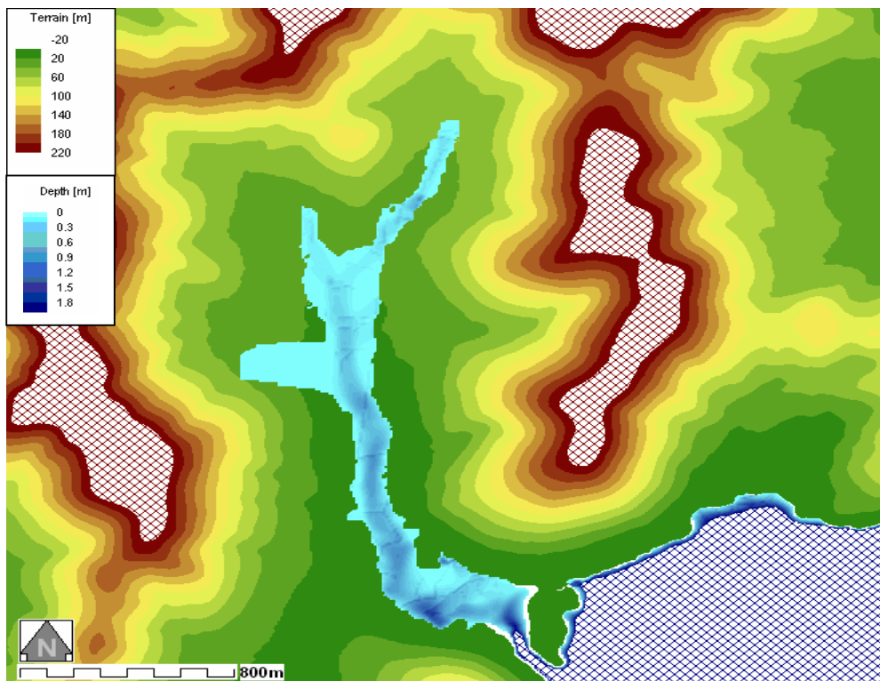
Figure 14: Water depth-Smooth with Roads_DTM10_M30 in Terrain map
