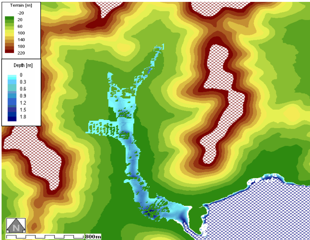
Figure 18: Water depth-Smooth with Roads and Buildings_DTM10_M20 in Terrain map
