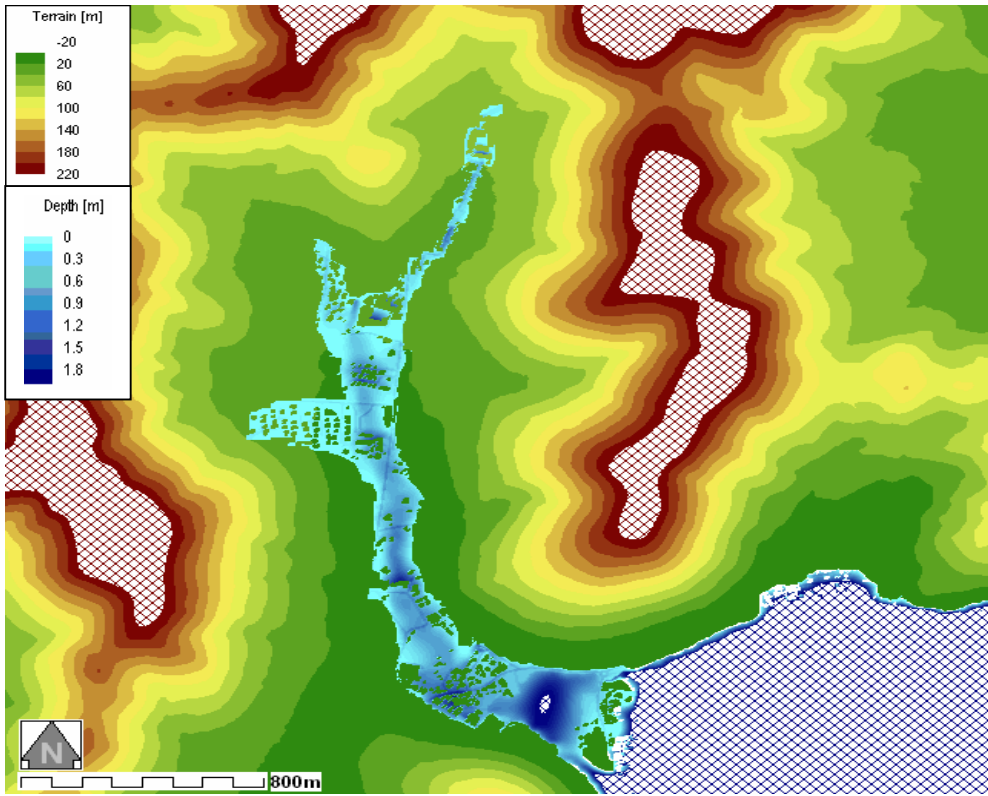
Figure 17: Water depth-Smooth with Roads and Buildings_DTM5_M20 in Terrain map
