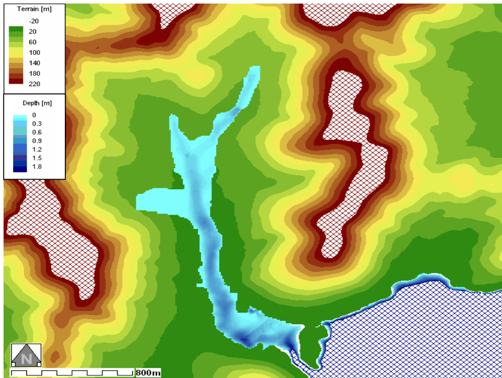
Figure 2: Water depth-Smooth DTM10_M20 in Terrain map
