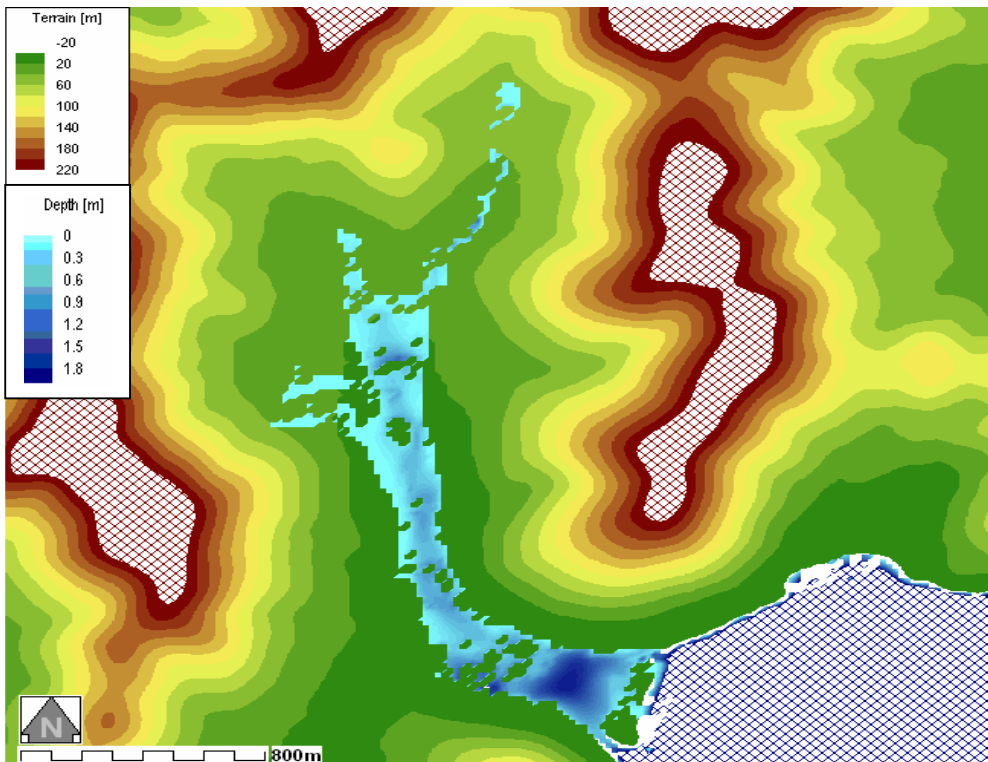
Figure 24: Water depth-Smooth with Roads and Buildings_DTM20_M30 in Terrain map
