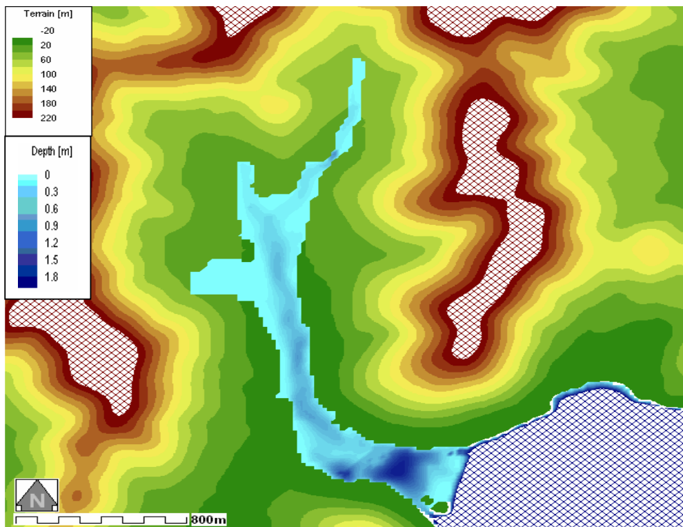
Figure 8: Water depth-Smooth DTM20_M30 in Terrain map
