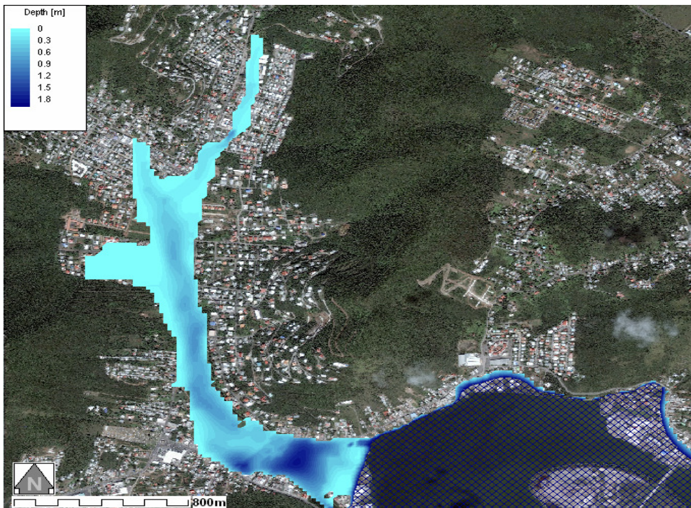
Figure 4: Water depth-Smooth DTM20_M20 Aerial Photo
