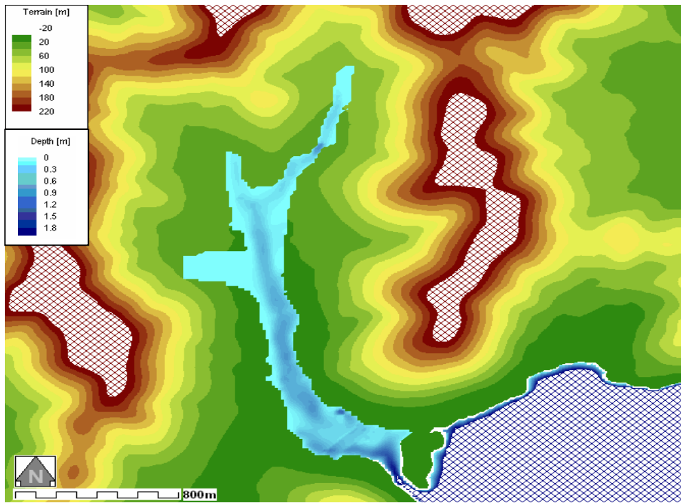
Figure 3: Water depth-Smooth DTM15_M20 in Terrain map
