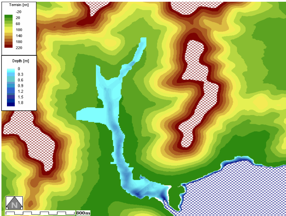
Figure 6: Water depth-Smooth DTM10_M30 in Terrain map
