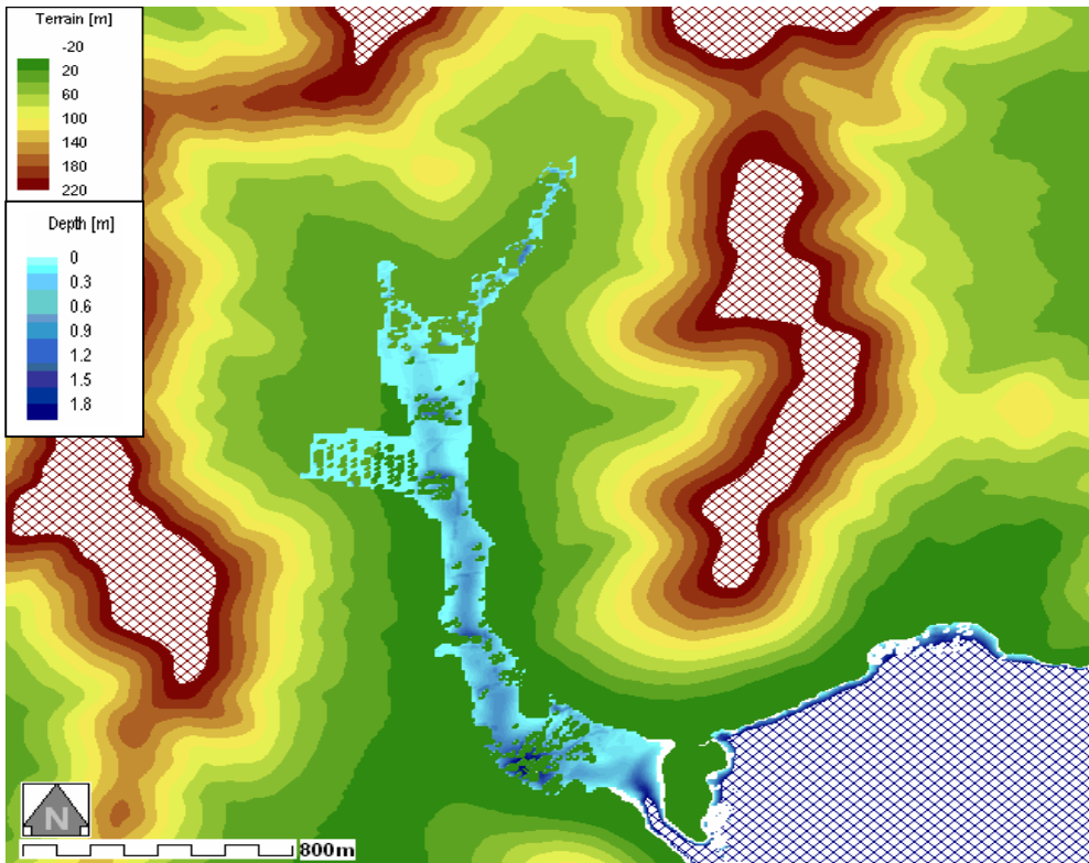
Figure 22: Water depth-Smooth with Roads and Buildings_DTM10_M30 in Terrain map
