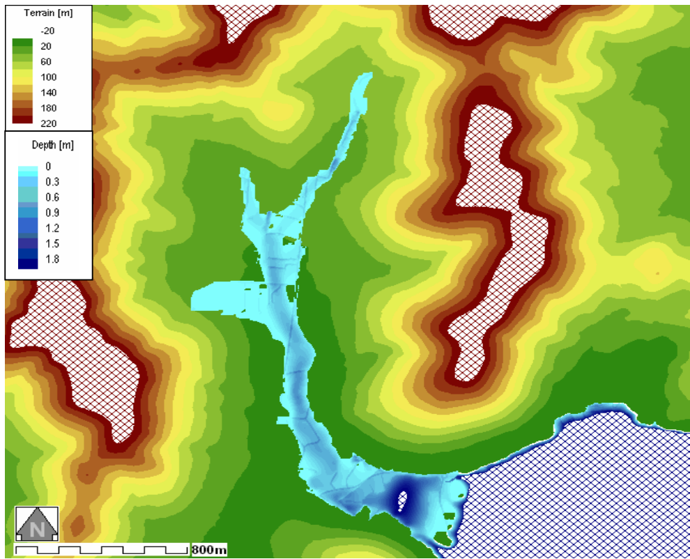
Figure 13: Water depth-Smooth with Roads_DTM5_M30 in Terrain map
