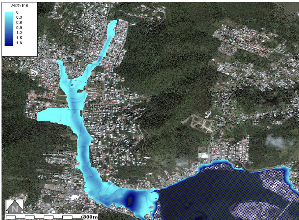
Figure 9: Water depth-Smooth with Roads DTM5_M20 Aerial Photo
