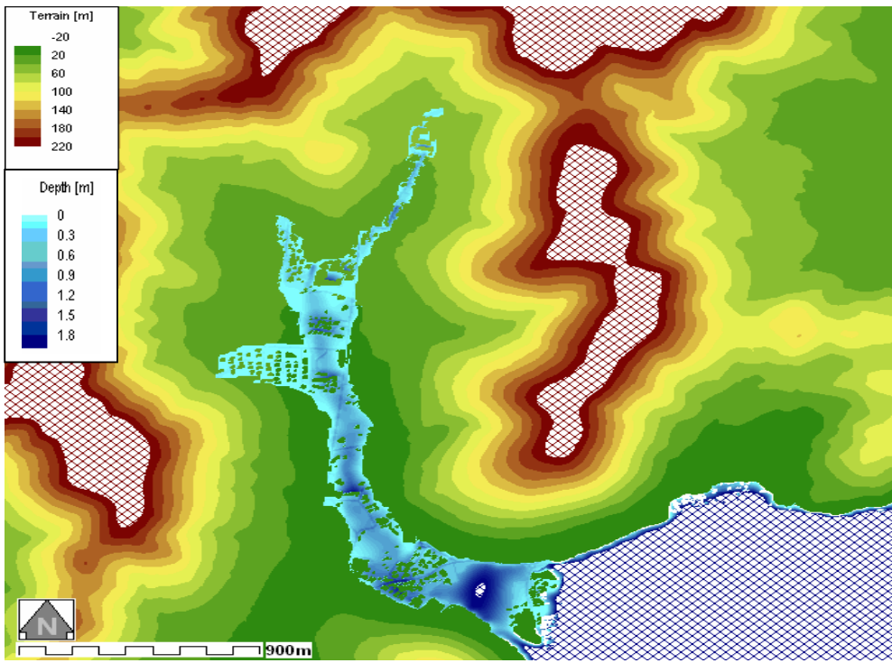
Figure 21: Water depth-Smooth with Roads and Buildings_DTM5_M30 in Terrain map
