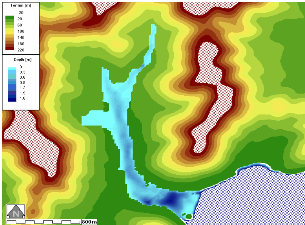
Figure 4: Water depth-Smooth DTM20_M20 in Terrain map
