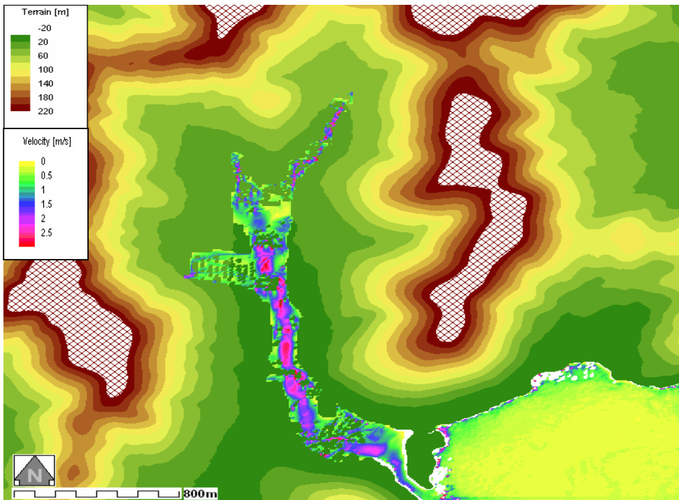
Figure 22: Flow velocity-Smooth with Roads and Buildings DTM10_M30 in Terrain map
