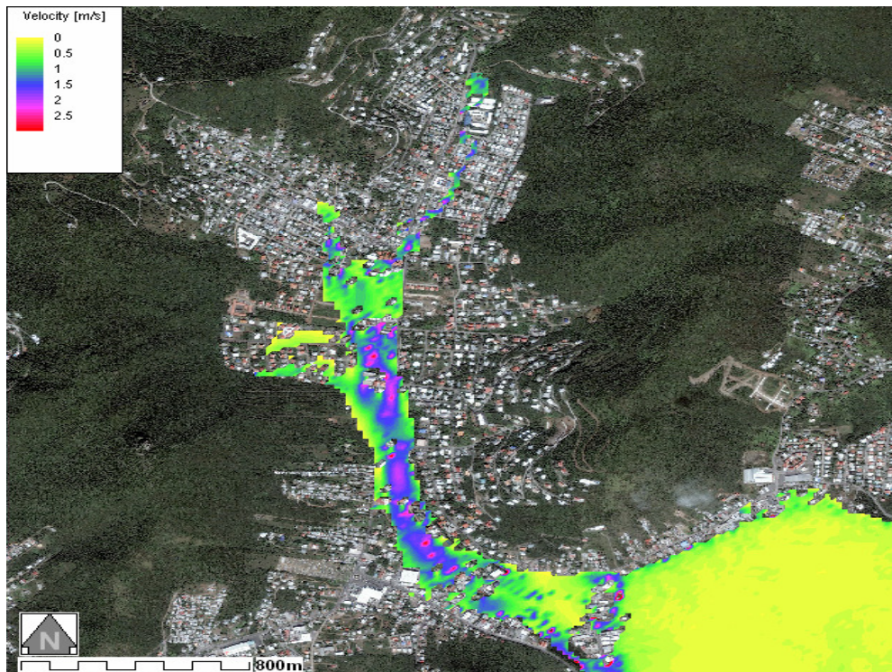
Figure 20: Flow velocity-Smooth with Road and Buildings_ DTM20_M20 Aerial Photo
