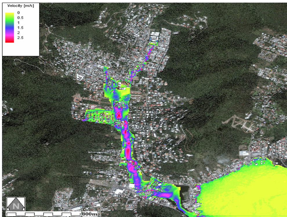
Figure 22: Flow velocity-Smooth with Road and Buildings_ DTM10_M30 Aerial Photo
