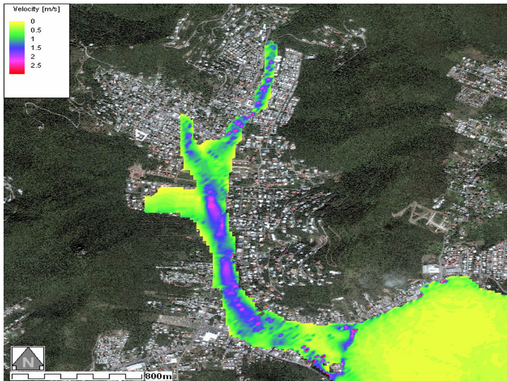
Figure 12: Flow velocity-Smooth with Roads DTM20_M20 Aerial Photo
