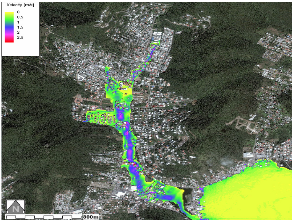
Figure 18: Flow velocity-Smooth with Road and Buildings_ DTM10_M20 Aerial Photo
