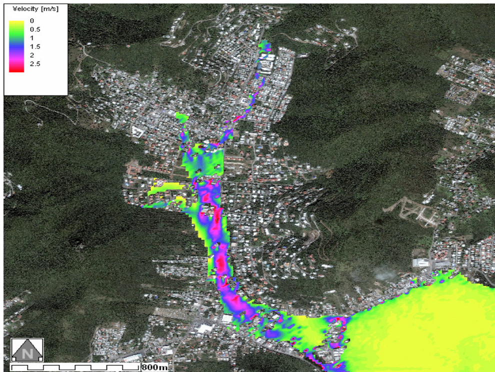
Figure 24: Flow velocity-Smooth with Road and Buildings_ DTM20_M30 Aerial Photo
