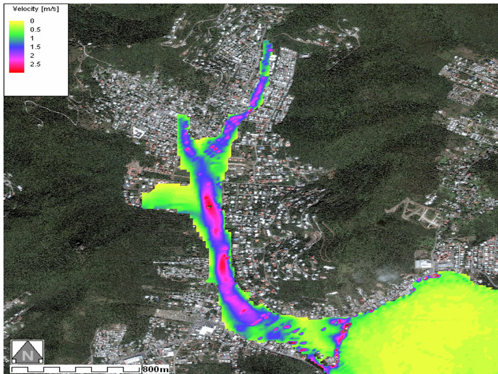
Figure 8: Flow velocity-Smooth DTM20_M30 Aerial Photo
