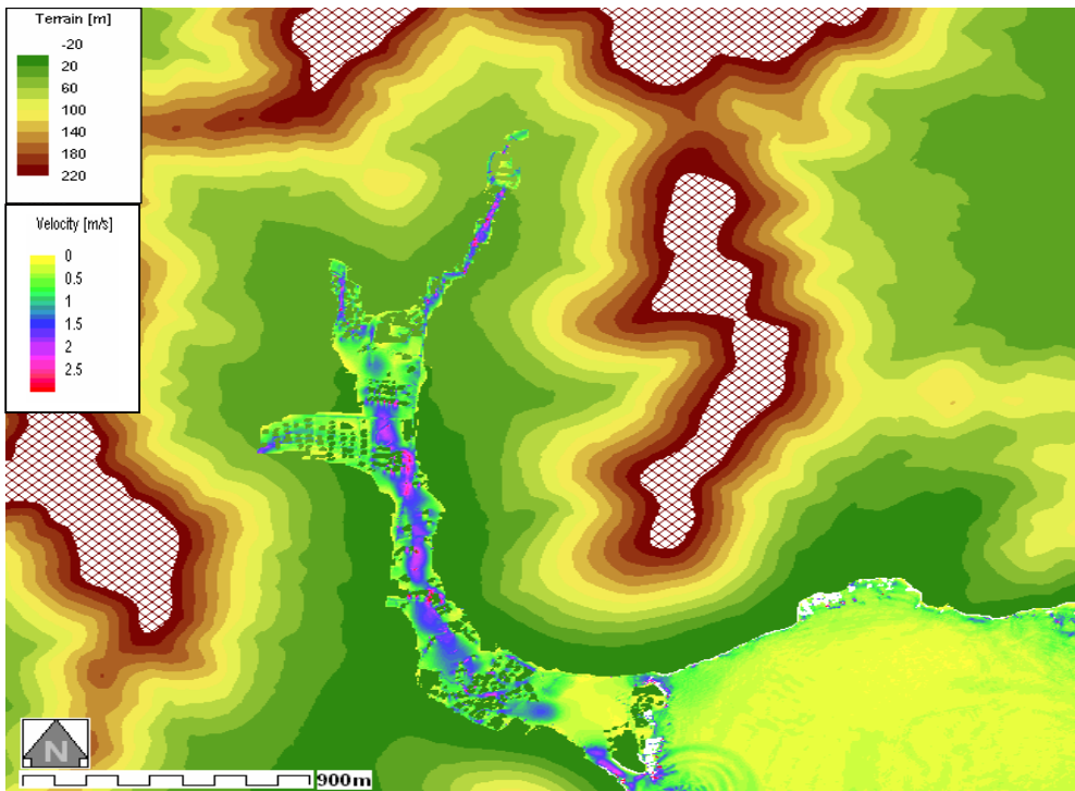
Figure 21: Flow velocity-Smooth with Roads and Buildings DTM5_M30 in Terrain map
