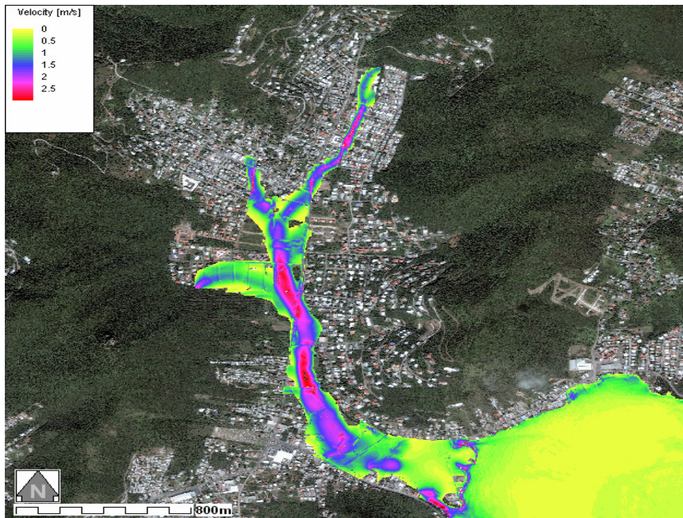
Figure 13: Flow velocity-Smooth with Roads DTM5_M30 Aerial Photo
