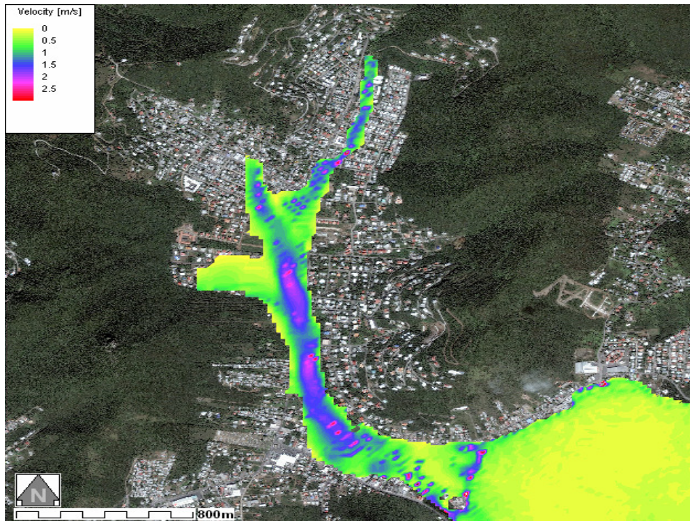
Figure 4: Flow velocity-Smooth DTM20_M20 Aerial Photo
