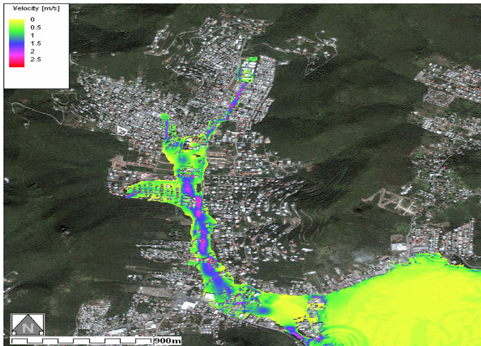
Figure 21: Flow velocity-Smooth with Road and Buildings_ DTM5_M30 Aerial Photo
