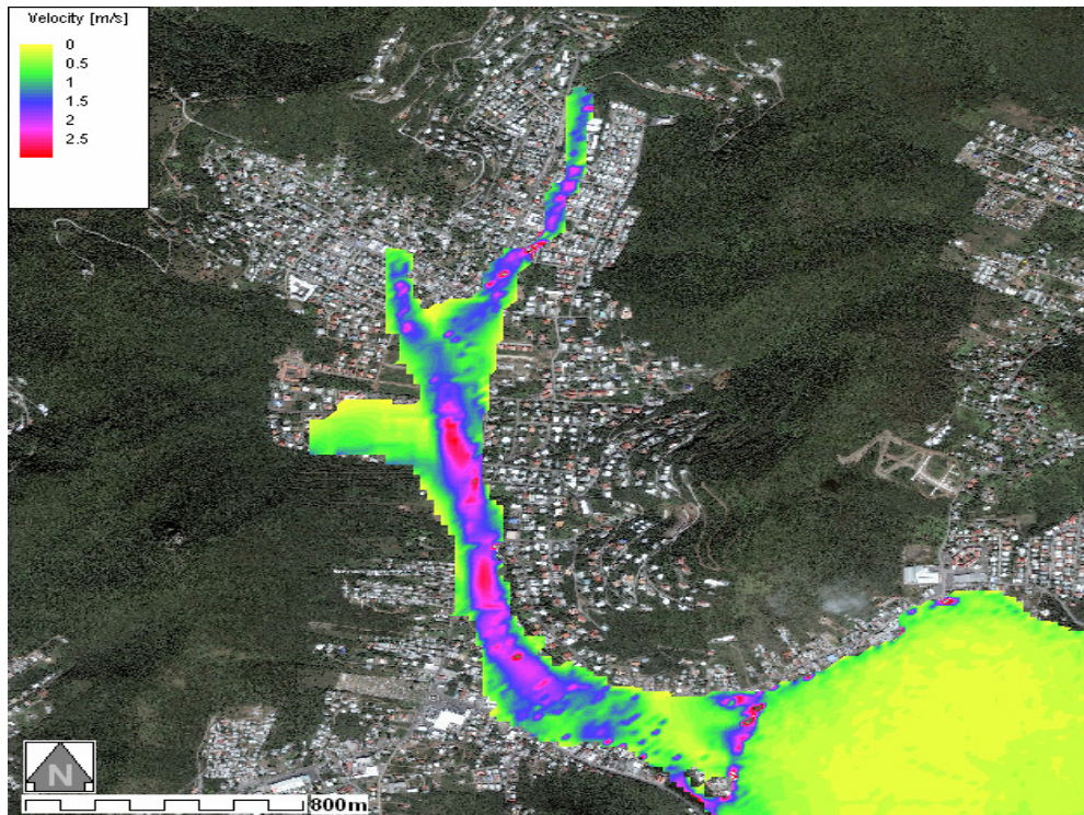
Figure 16: Flow velocity-Smooth with Roads DTM20_M30 Aerial Photo
