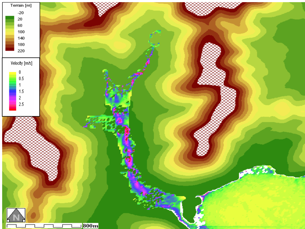
Figure 23: Flow velocity-Smooth with Roads and Buildings DTM15_M30 in Terrain map
