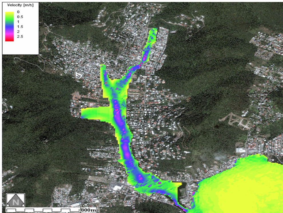
Figure 11: Flow velocity-Smooth with Roads DTM15_M20 Aerial Photo
