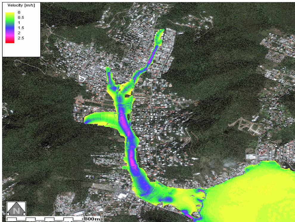
Figure 9: Flow velocity-Smooth with Roads DTM5_M20 Aerial Photo
