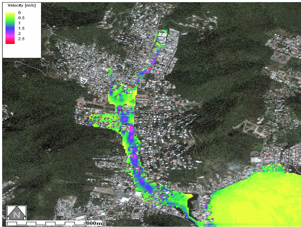
Figure 19: Flow velocity-Smooth with Road and Buildings_ DTM15_M20 Aerial Photo
