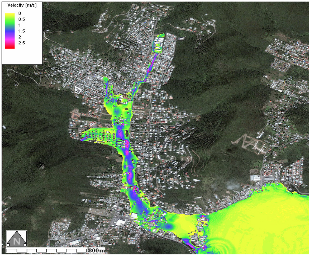
Figure 17: Flow velocity-Smooth with Road and Buildings_ DTM5_M20 Aerial Photo
