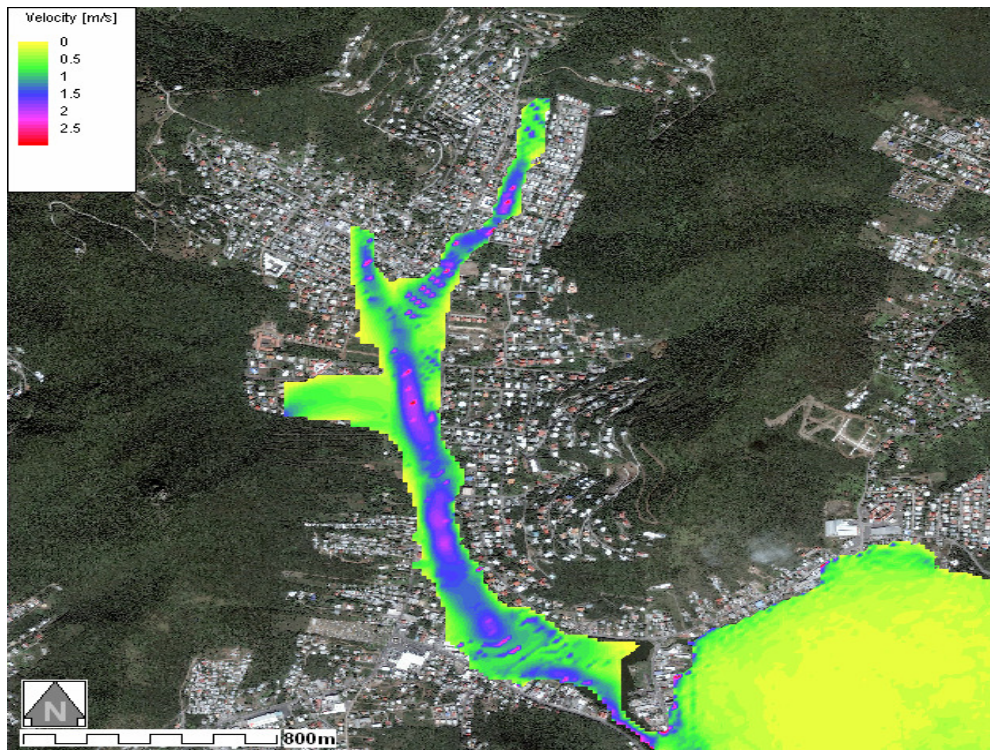
Figure 3: Flow velocity-Smooth DTM15_M20 Aerial Photo
