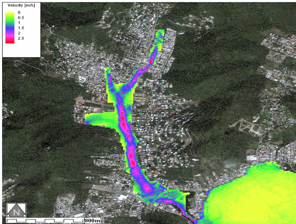
Figure 15: Flow velocity-Smooth with Roads DTM15_M30 Aerial Photo
