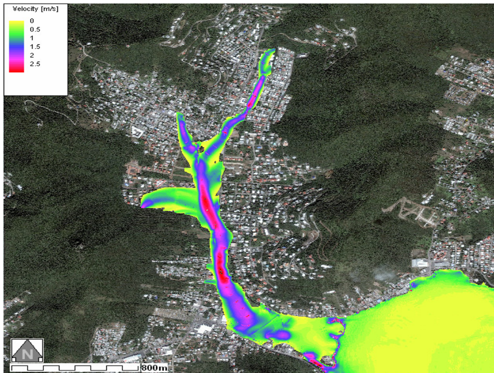
Figure 5: Flow velocity-Smooth DTM5_M30 Aerial Photo
