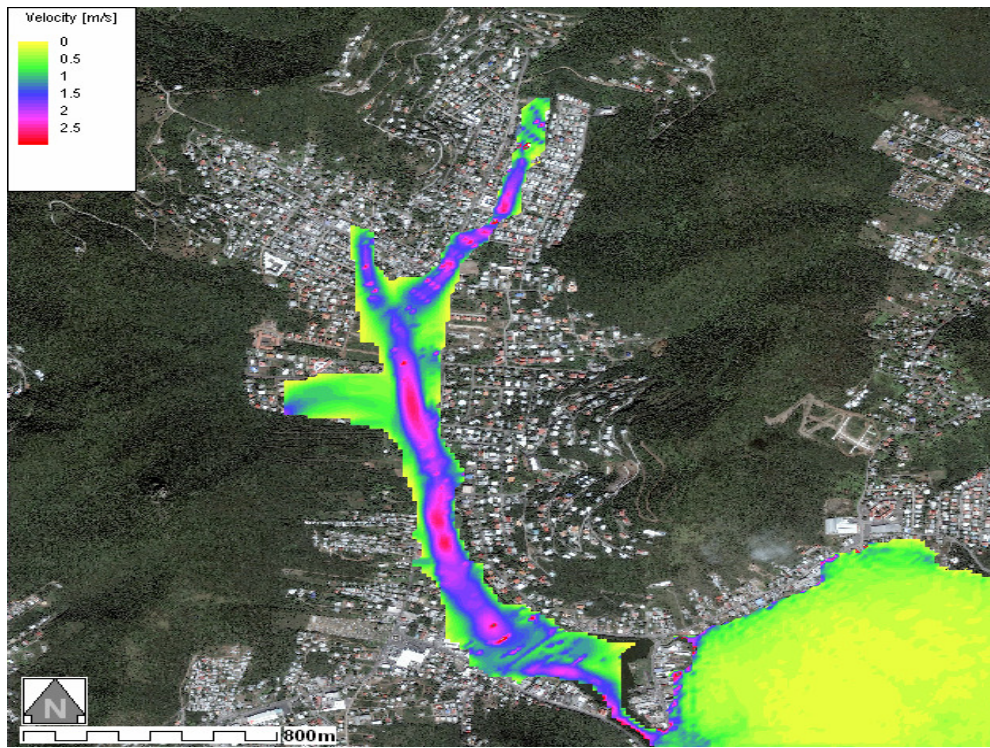
Figure 7: Flow velocity-Smooth DTM15_M30 Aerial Photo
