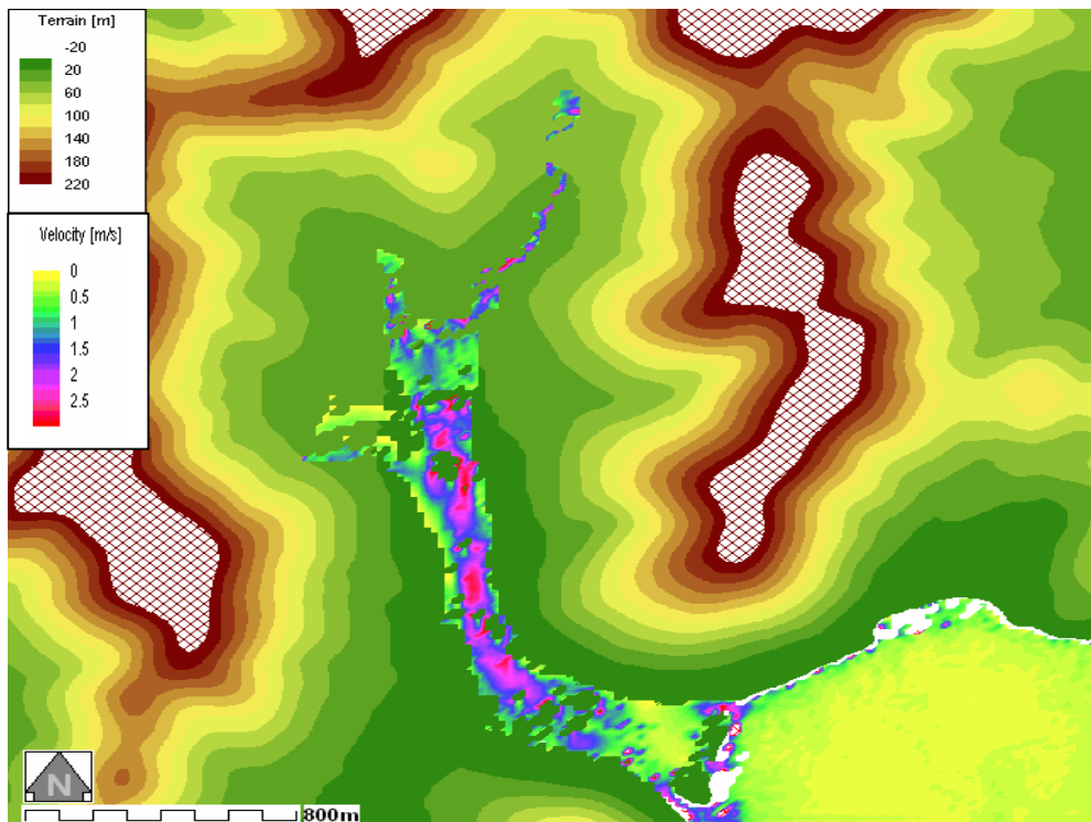
Figure 24: Flow velocity-Smooth with Roads and Buildings DTM20_M30 in Terrain map
