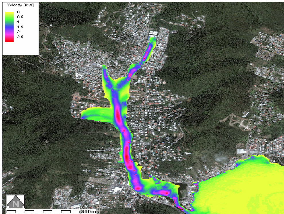
Figure 6: Flow velocity-Smooth DTM10_M30 Aerial Photo
