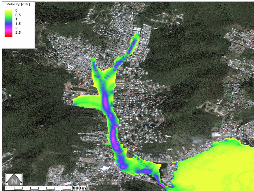
Figure 2: Flow velocity-Smooth DTM10_M20 Aerial Photo
