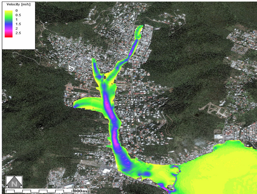
Figure 1: Flow velocity-Smooth DTM5_M20 Aerial Photo
