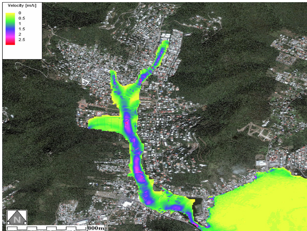
Figure 10: Flow velocity-Smooth with Roads DTM10_M20 Aerial Photo
