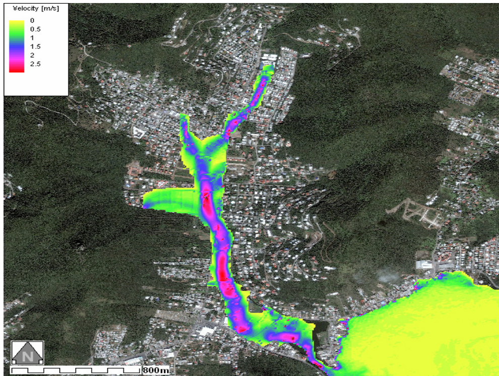
Figure 14: Flow velocity-Smooth with Roads DTM10_M30 Aerial Photo
