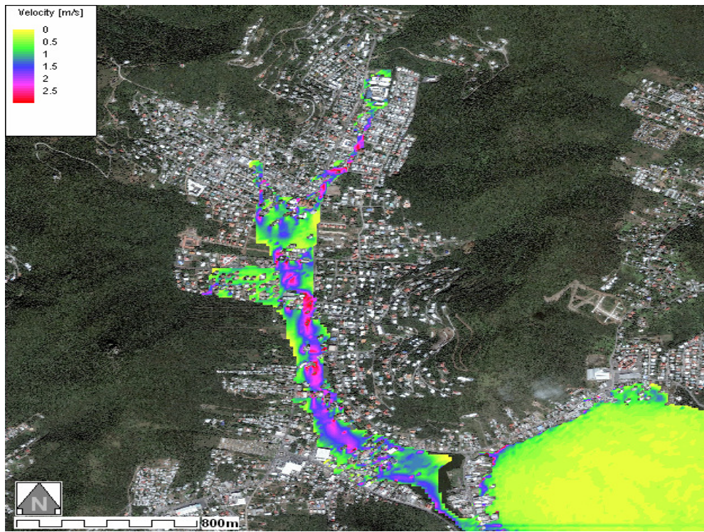
Figure 23: Flow velocity-Smooth with Road and Buildings_ DTM15_M30 Aerial Photo
