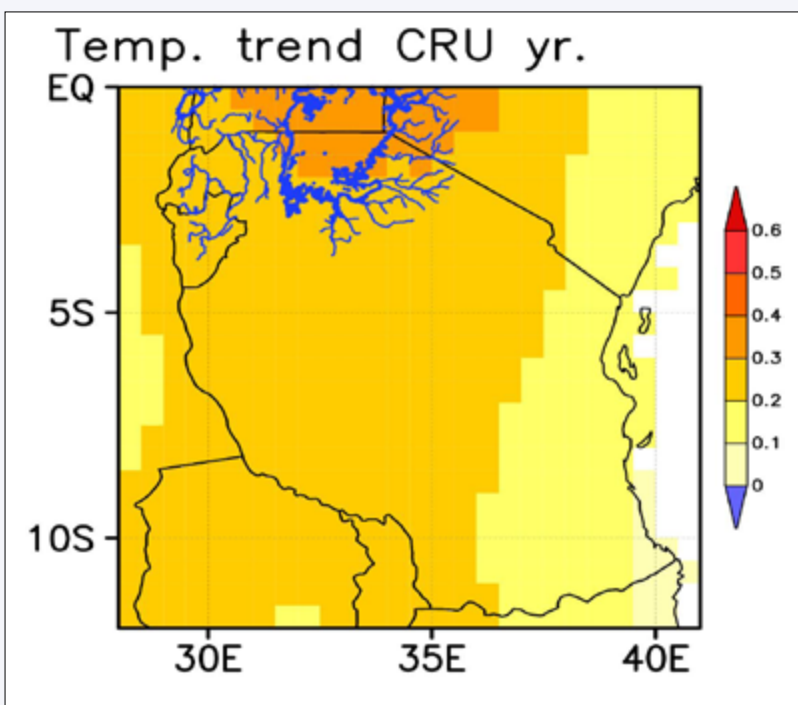
Figure 4: The monotonic slope in temperature (deg C) between 1963 and 2012 at each grid cell, according to a linear trend per decade for Jan to Dec. Hatching indicates areas where the trend is not statistically significant at the 95% level. Data taken from the CRU TS3.22 datasets.
