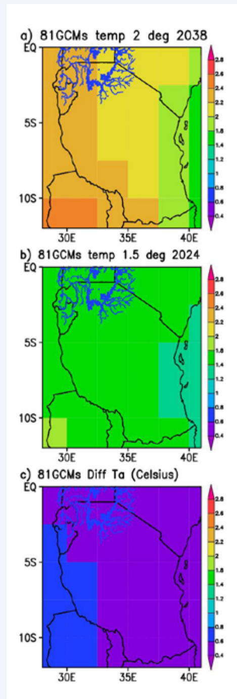
Figure 6: Projected spatial annual temperature change for Tanzania, at the time of global warming level of 2°C, 1.5 °C, and the difference. Data are average from 81 CMIP5 climate model simulations under the RCP8.5 forcing scenario.
