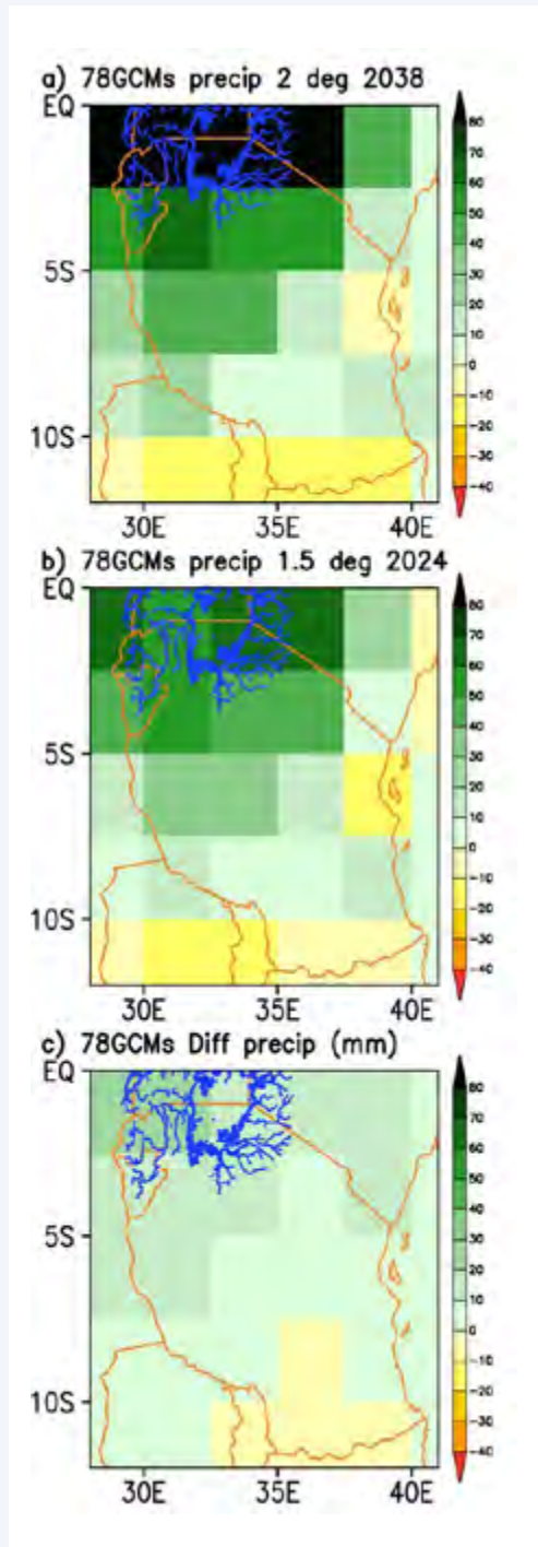
Figure 5: Projected spatial annual rainfall change for Tanzania, at the time of global warming of 2°C, 1.5 °C, and the difference. Data are average from 78 CMIP5 climate model simulations under the RCP8.5 forcing scenario.
