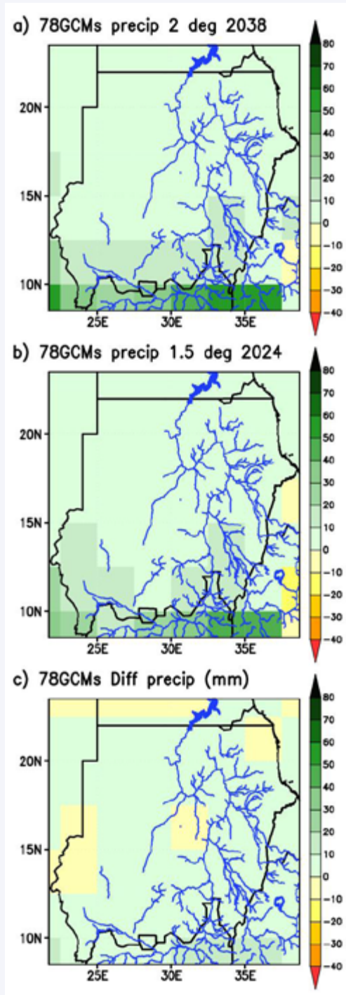
Figure 5: Projected spatial annual rainfall change for Sudan, at the time of global warming of 2°C, 1.5 °C, and the difference. Data are average from 78 CMIP5 climate model simulations under the RCP8.5 forcing scenario.
