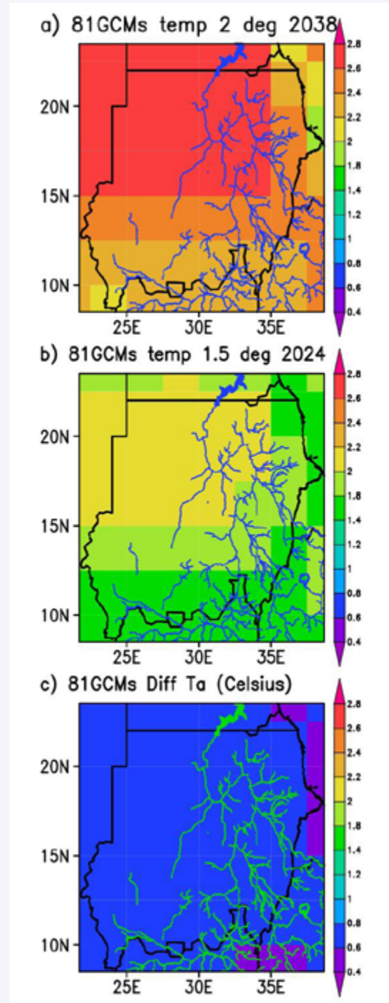
Figure 6: Projected spatial annual temperature change for Sudan, at the time of global warming level of 2°C, 1.5 °C, and the difference. Data are average from 81 CMIP5 climate model simulations under the RCP8.5 forcing scenario.
