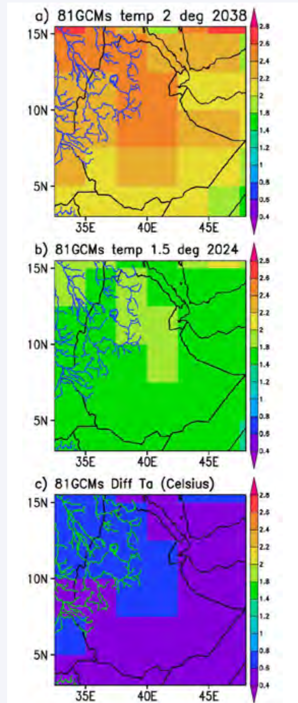
Figure 6: Projected spatial annual temperature change for Ethiopia, at the time of global warming level of 2°C, 1.5 °C, and the difference. Data are average from 81 CMIP5 climate model simulations under the RCP8.5 forcing scenario.
