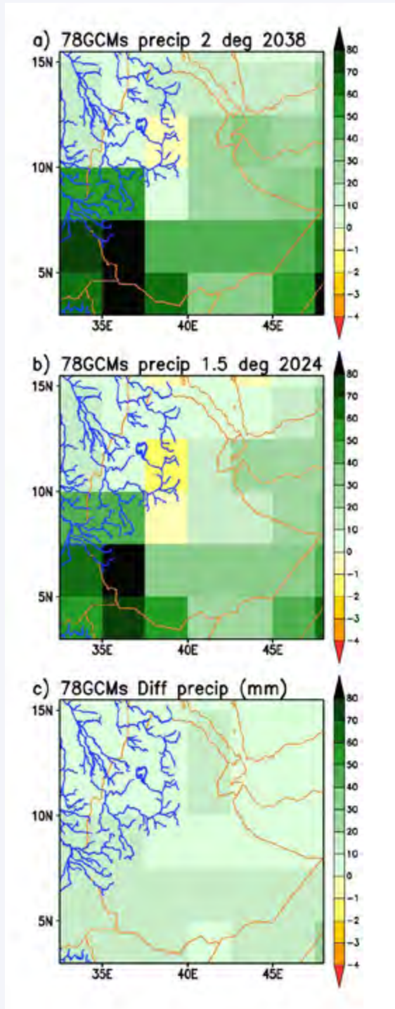
Figure 5: Projected spatial annual rainfall change for Ethiopia, at the time of global warming of 2°C, 1.5 °C, and the difference. Data are average from 78 CMIP5 climate model simulations under the RCP8.5 forcing scenario.
