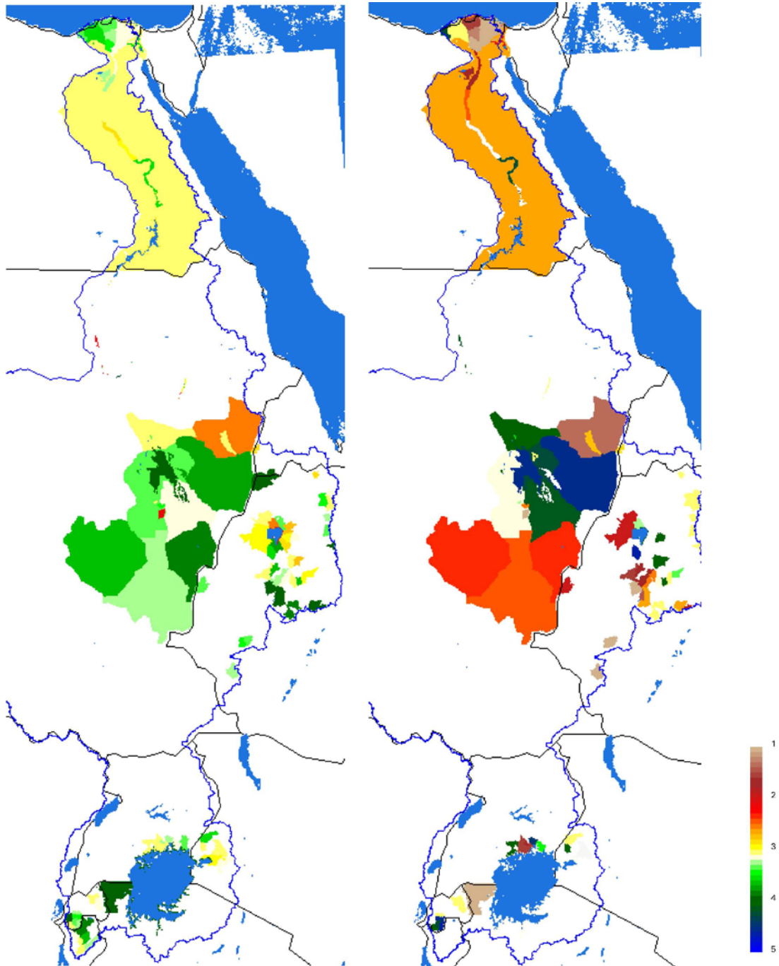
Land and crop sustainability Water resources sustainability Figure 18 Spatial variation of the sustainability of irrigation systems in the Nile Basin across all administrative districts. The value is expressed as a score between 1 (very poor) to 5 (excellent). The Nile Valley has a larger administrative unit with pockets of irrigation at the fringes with the Nile Delta
