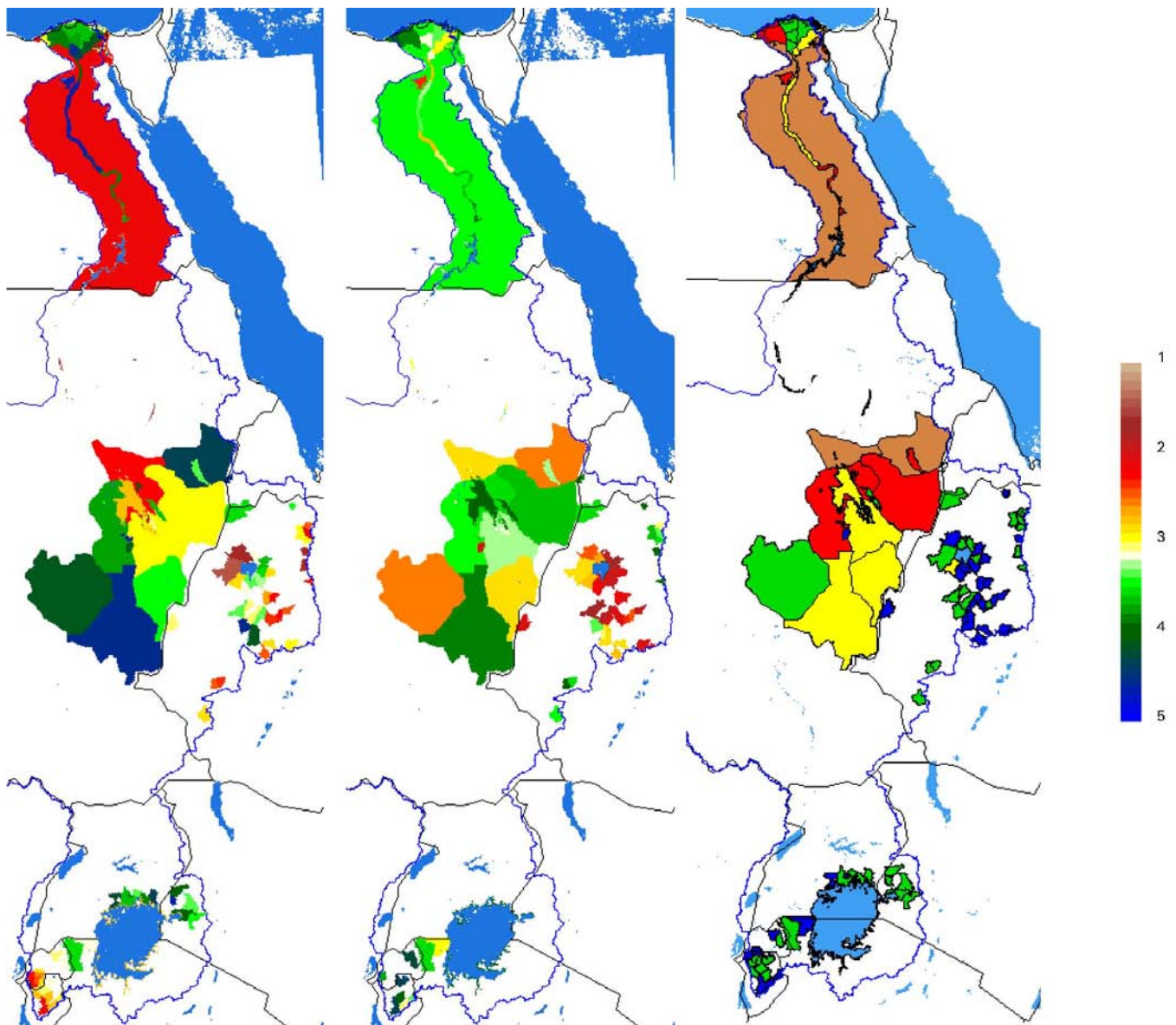
Crop water consumption Crop water deficit Adequacy
