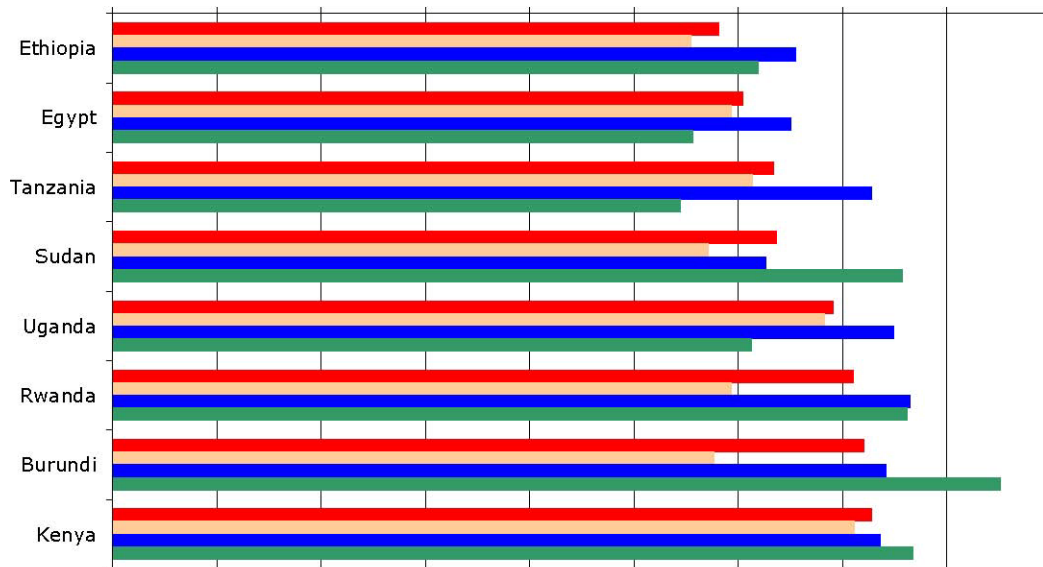
Figure 21 Breakdown of the average irrigation performance scores ( RO, PO, and SO and their average values) by country in the Nile Basin
