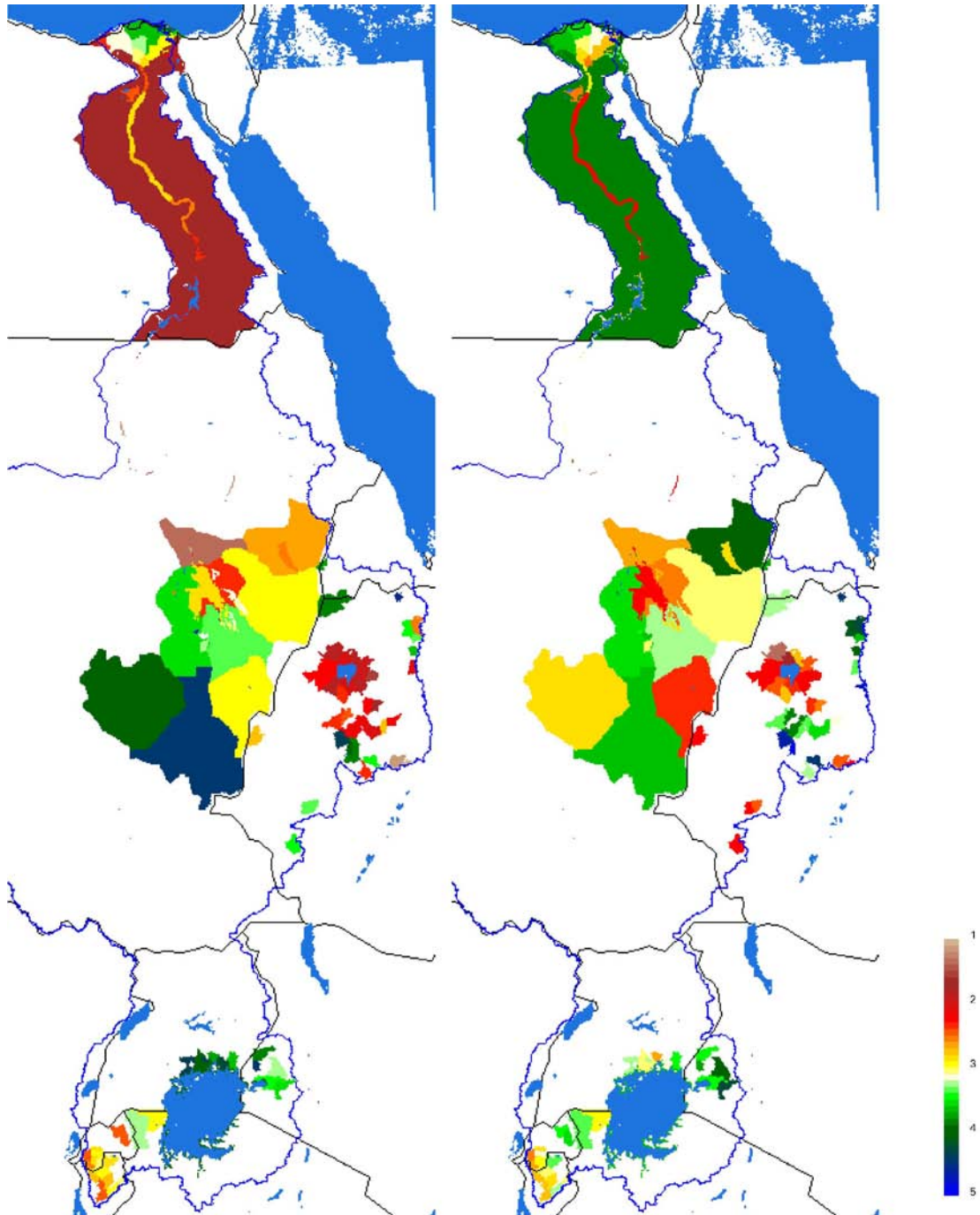
Land productivity (-) Water productivity (-) Figure 17 Spatial variation of the land and water productivity in the Nile Basin across all administrative districts based on remote sensing data. The value is expressed as a score between 1 (very poor) to 5 (excellent). The Nile Valley has a larger administrative unit with pockets of irrigation at the fringes with the Nile Delta
