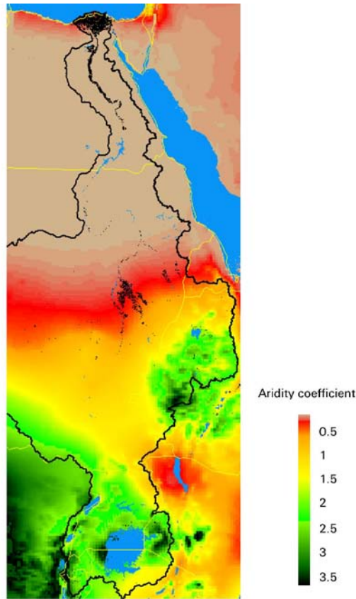
Figure 14 Spatial patterns of rainfall/reference ET across the entire Nile basin to e differences. The irrigation mask is superimposed
