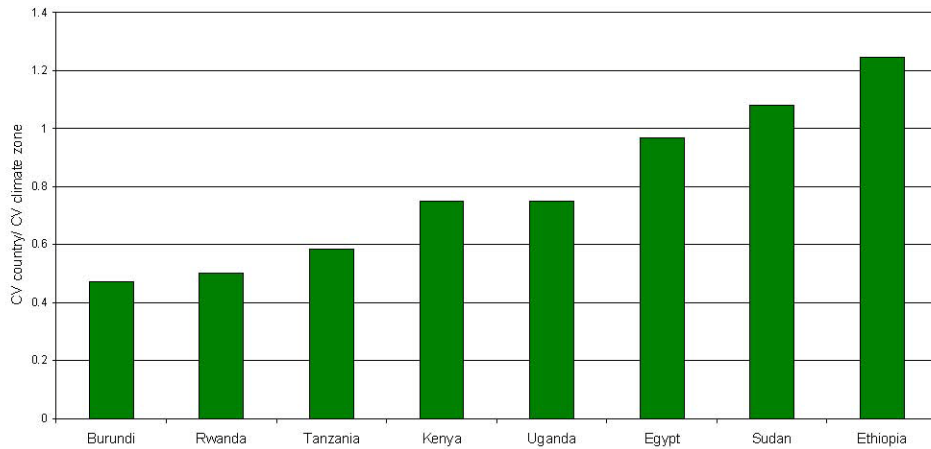
Figure 27 Impact of good water governance on the reduction of spatial variations of Result Oriented indicators (i.e. productivity) as compared to the prevailing climatic system
